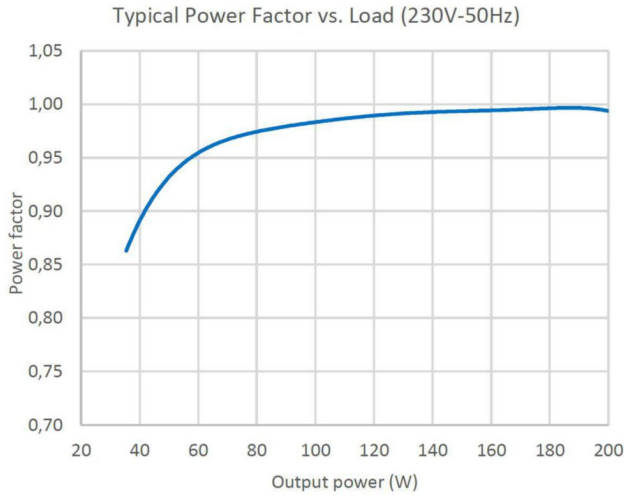
OT 200 1A0 4DIM NFC G3 Typical power factor vs Load
